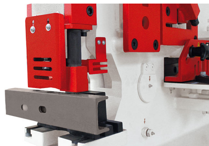
Notching station with safeguard
