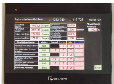
Dressing mode for grinding wheels with automatic dimension and speed (rpm) compensation ensures constant grinding rate and can be entered while in auto mode
