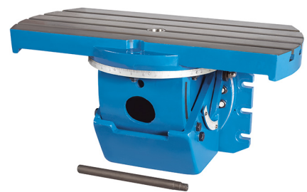
Universal swivel table for FPK 4.3/ FPK 6.3 (253721)
